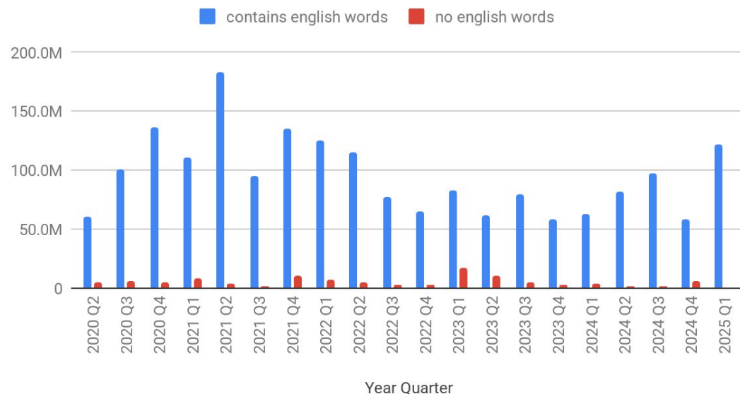
Contains english words and no english words
